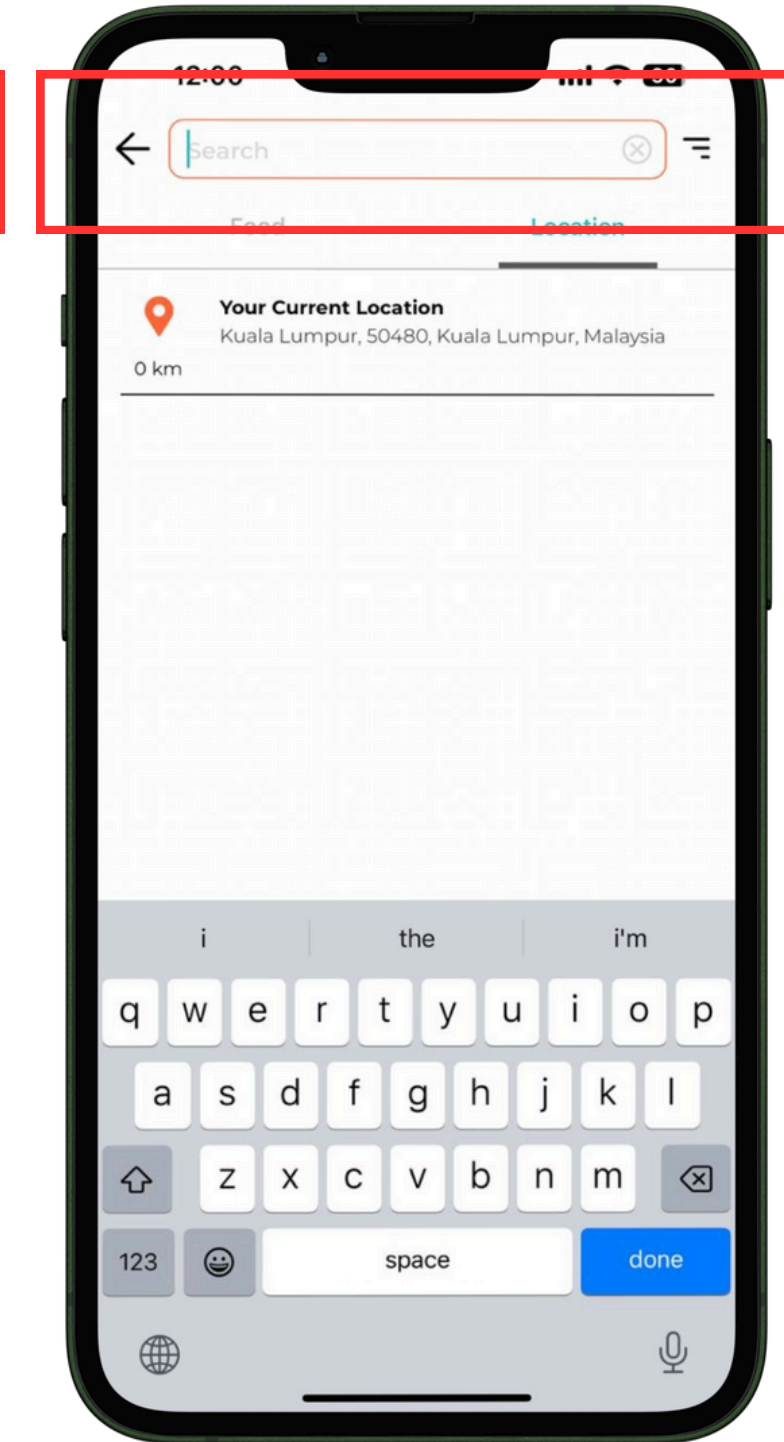
Live App
