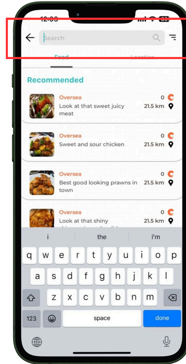
Live App
