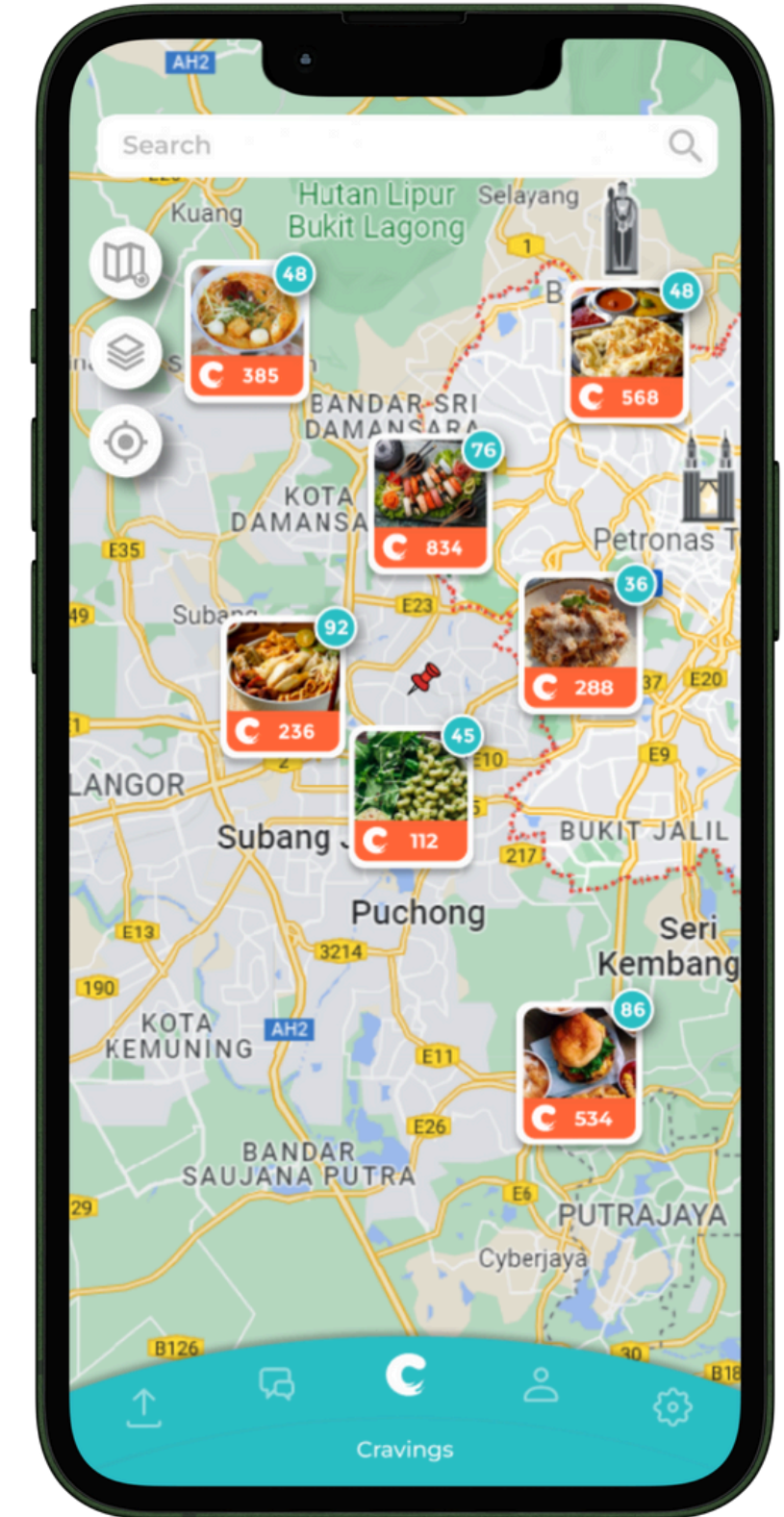
UI/UX Design
