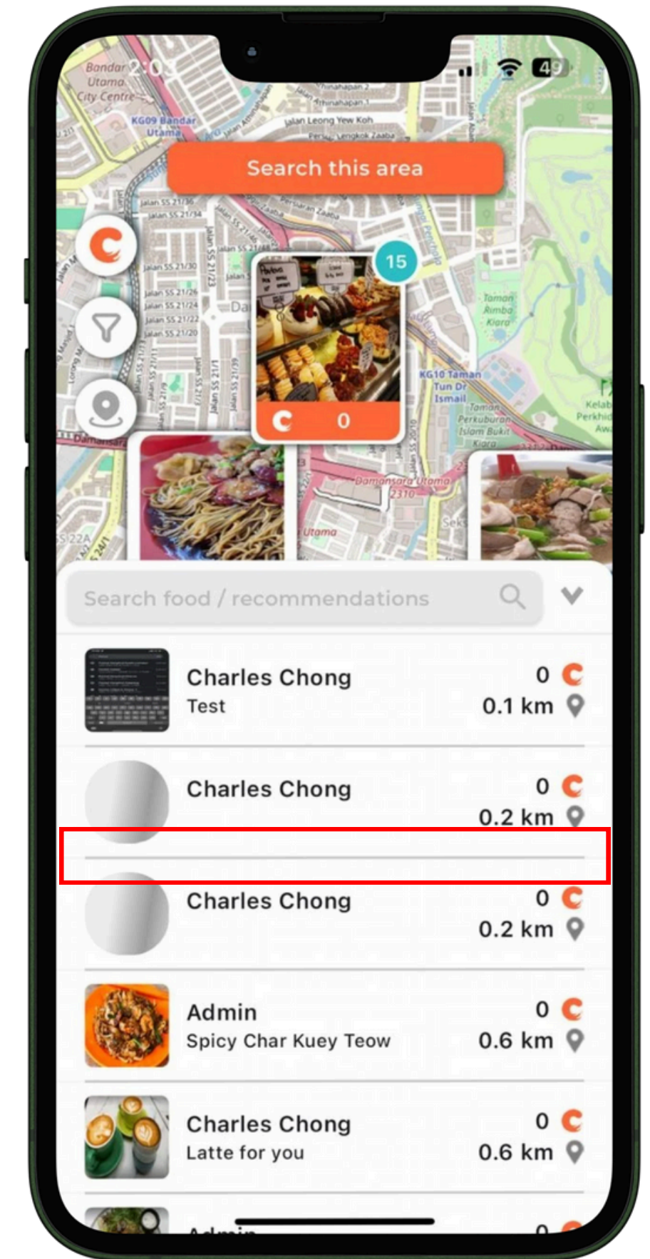
Live App
