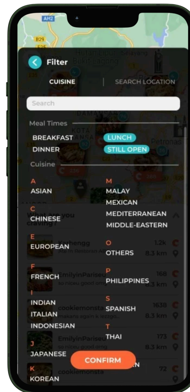
UI/UX Design
